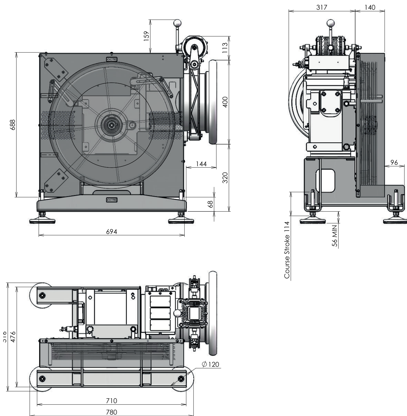
Machine MANGO 400 MH Horizontal gauche Horizontal left machine MANGO 400 for above machine room
