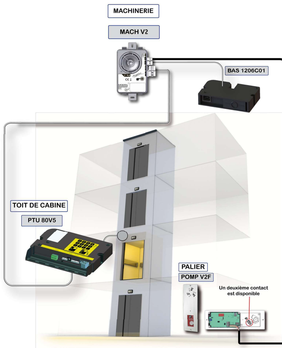
Figure 1. Câblage
